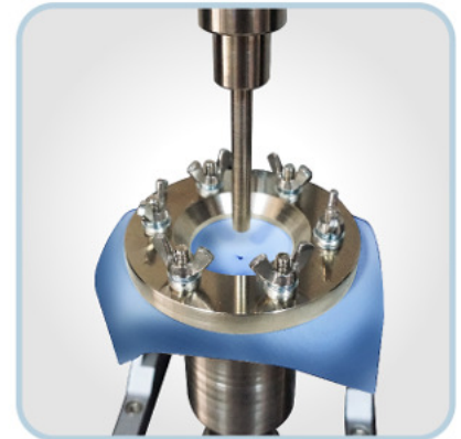
Puncture Test
